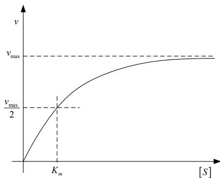
Figure 2: Michaelis-Menten diagram
