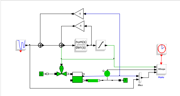
Figure 1: A mixed Scicos diagram including standard Scicos and Modelica blocks
