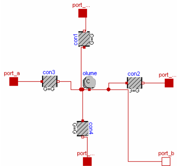
Figure 6: Structure of the PCM-Volume
