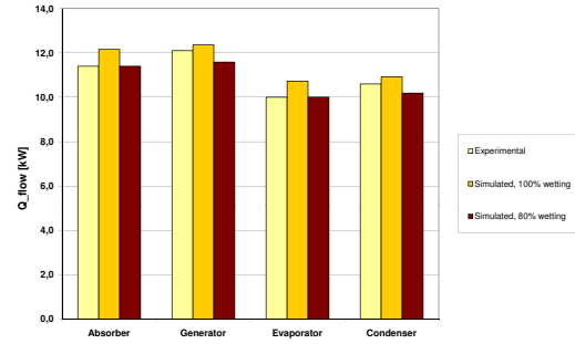
Figure 5: Stationary heat flow at nominal conditions
