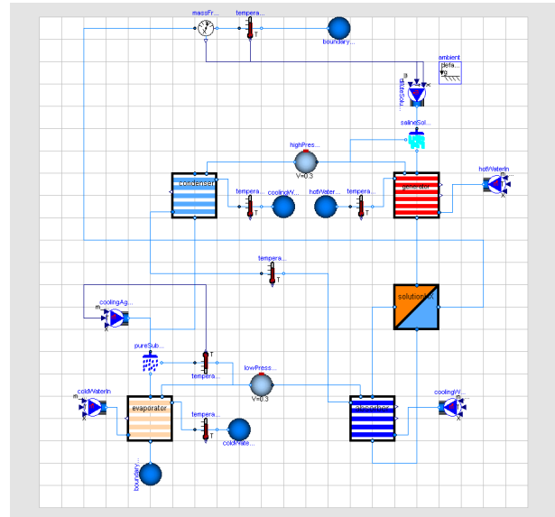
Figure 3: Diagramm of complete model
