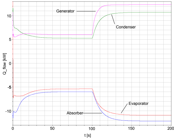
Figure 4: Response of external heat flows to step in driving temperature (55°C to 75°C at 100 s)
