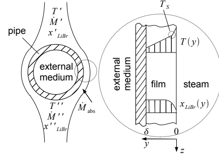
Figure 1: Schematic of a single absorber tube, concentration and temperature profile
