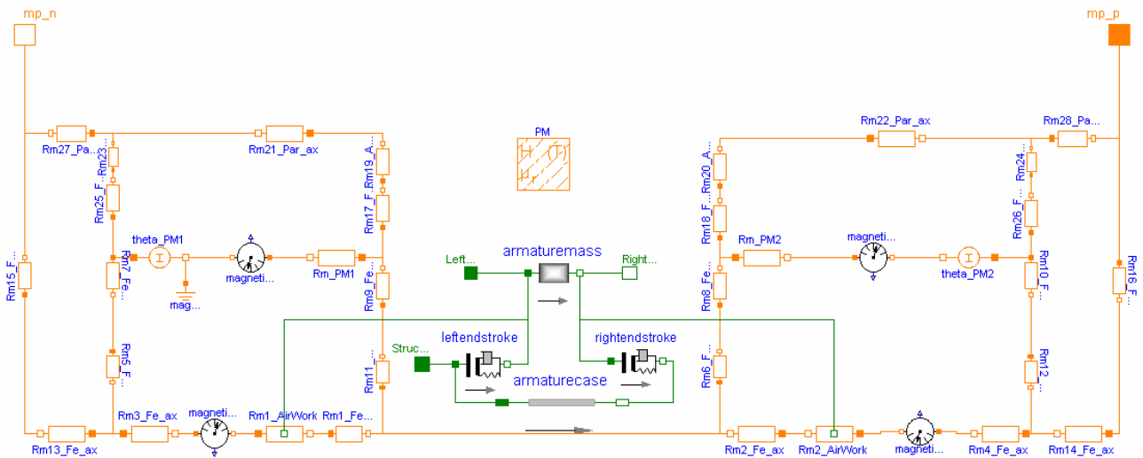
Figure 3 – Permanent magnet section of the motor model.
