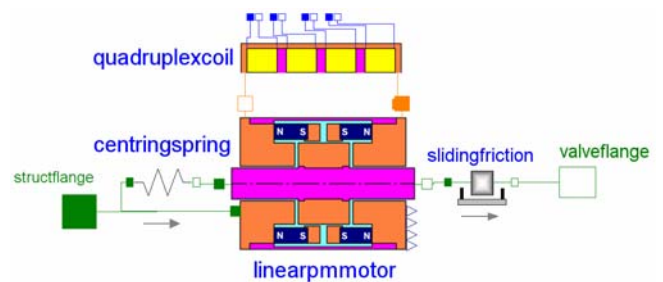
Figure 5 – Model of the fault-tolerant direct-drive motor.
